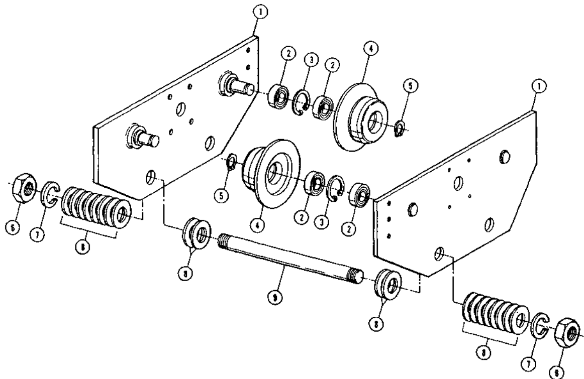
Figure 4. Push Type Rigid Mount Trolley Assembly — (4" \varnothing Wheels — 6" c/c Pins.) and Trailer Trolley * - (2 — 4" \varnothing Wheels).
