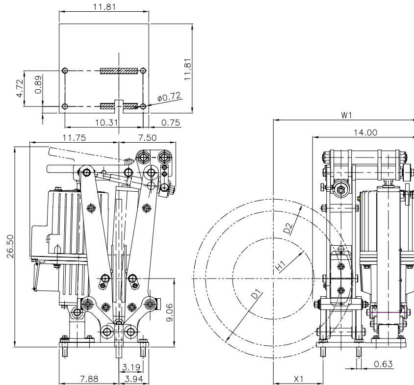
Standard brake designed for 3/4" disc thickness
