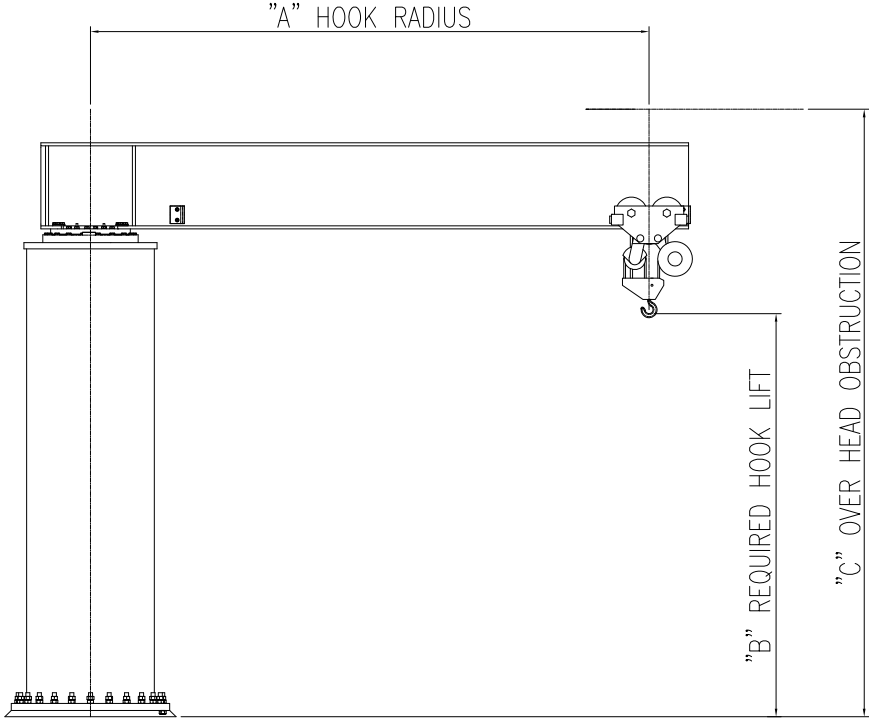
SINGLE GIRDER
