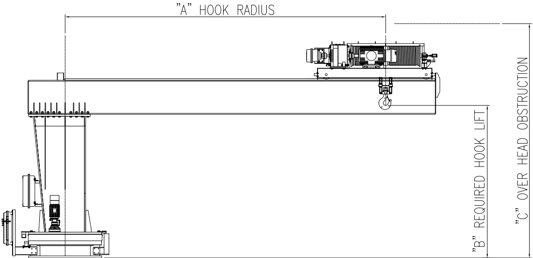
DOUBLE GIRDER
