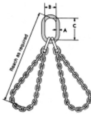
Basket Type Chain Sling ( Single & Double )
